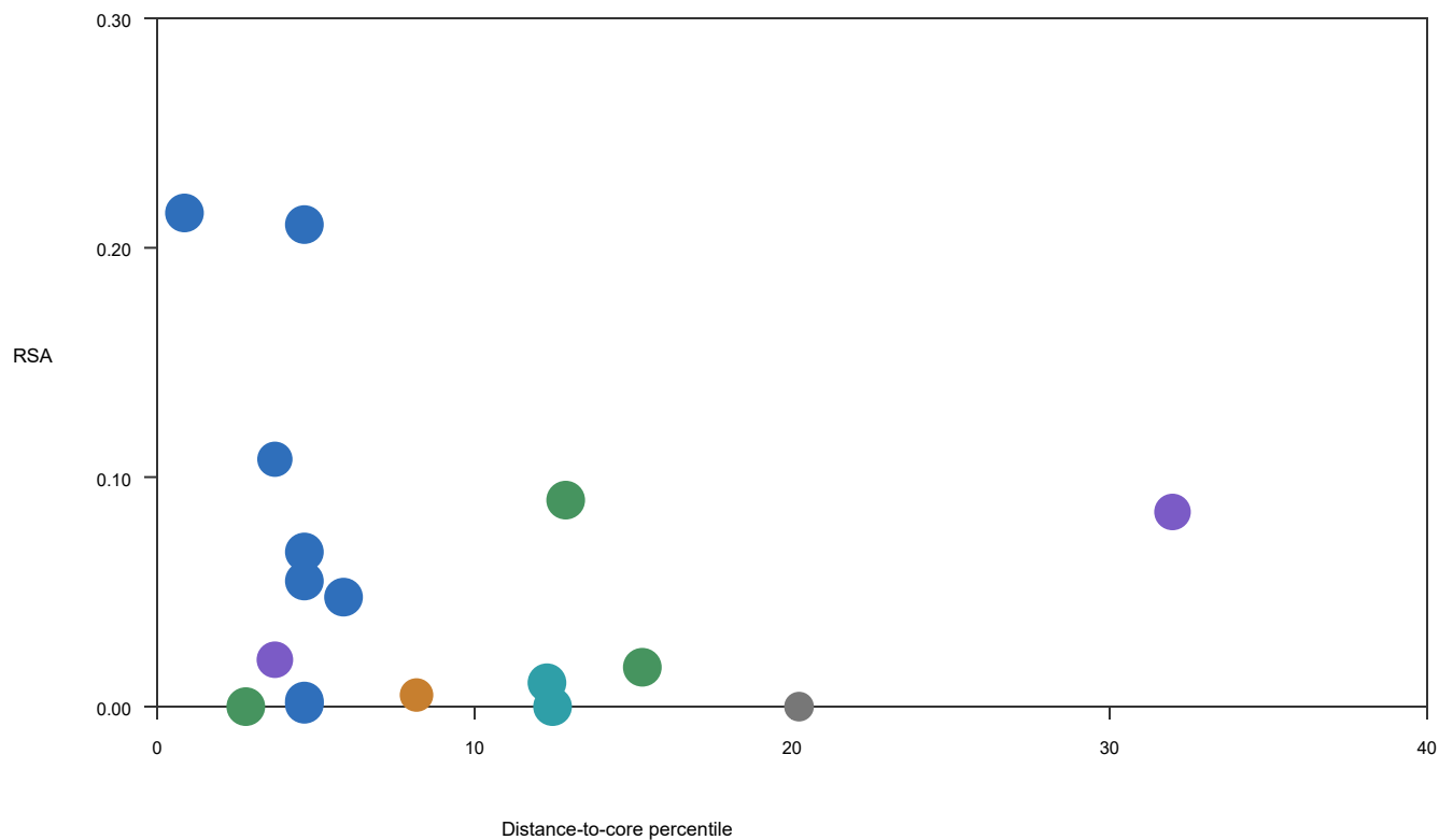
Figure 4. Distance percentile, RSA, and conservation annotations
