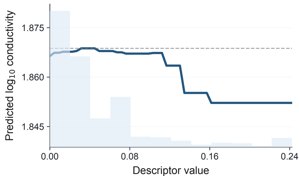
Hydration-overlap contrast
