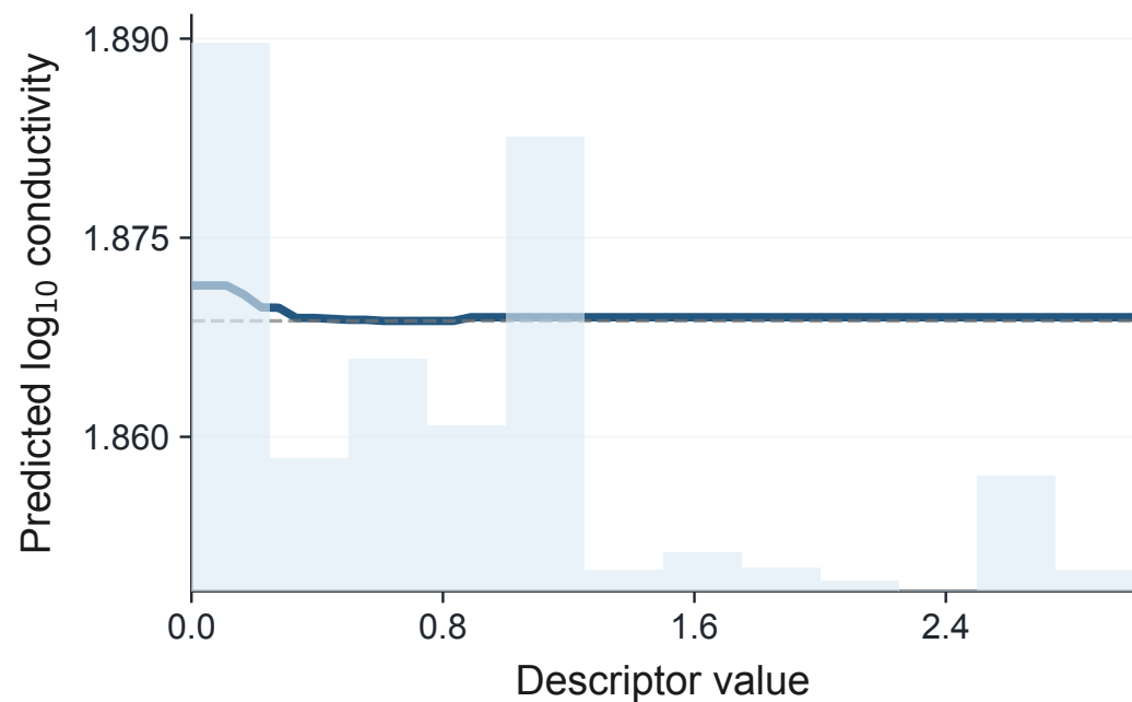
Spacer branching descriptor
