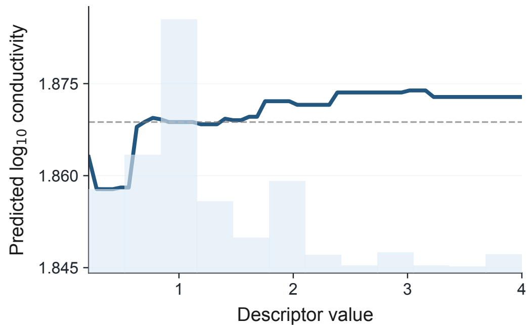
Cation count
