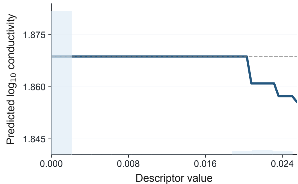
Sulfone motif density
