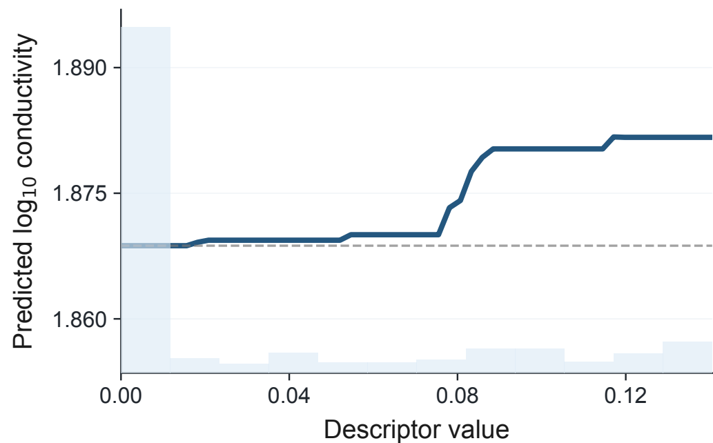
Fluorination
