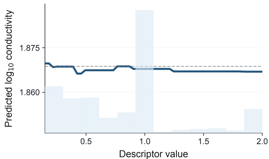
Cation-family count
