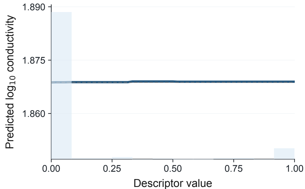
Pyrrolidinium-like fraction
