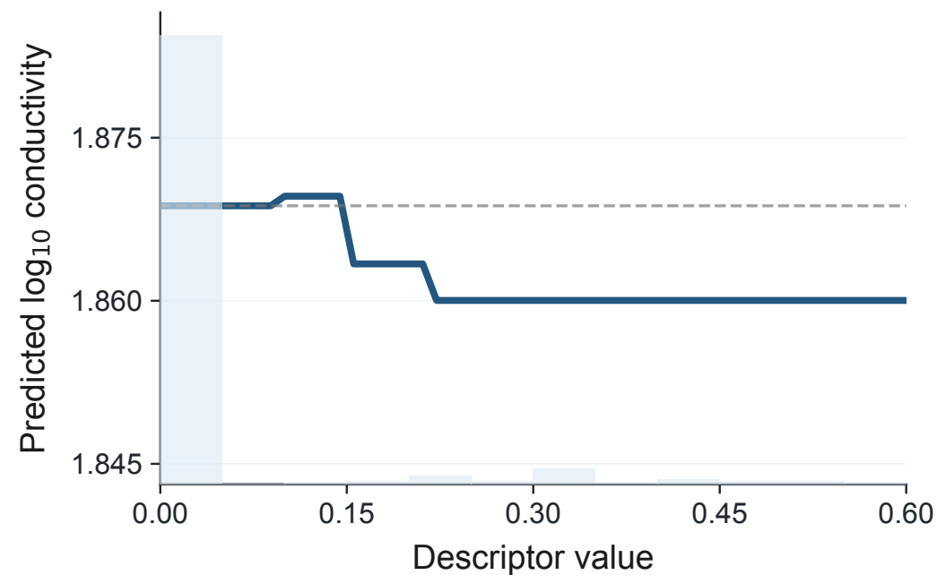
Imidazolium-like fraction
