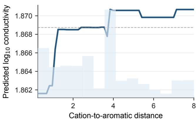
Cation-to-aromatic distance
