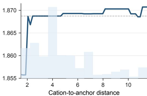
Cation-to-anchor distance
