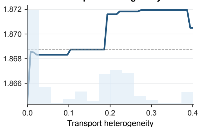
Transport heterogeneity
