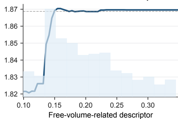
Free-volume-related descriptor
