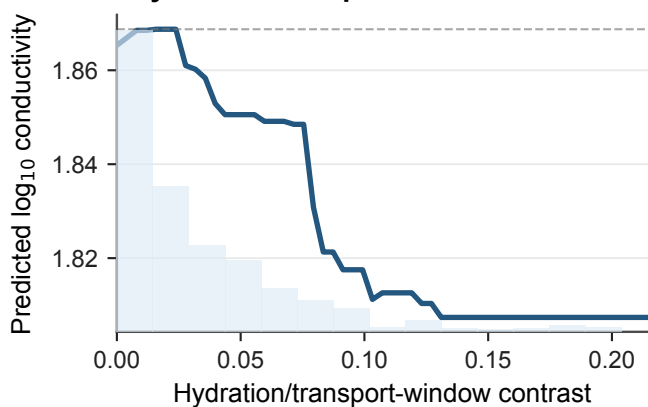
Hydration/transport-window contrast
