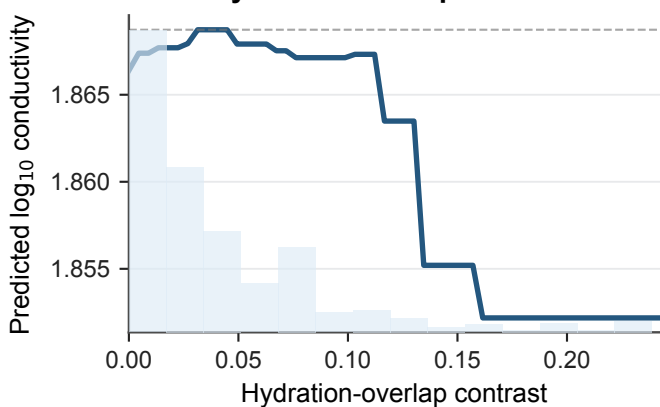
Hydration-overlap contrast
