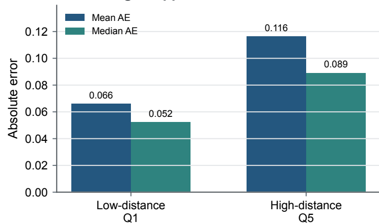
C Low vs high support
