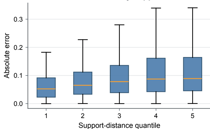
B Observation-level error by support
