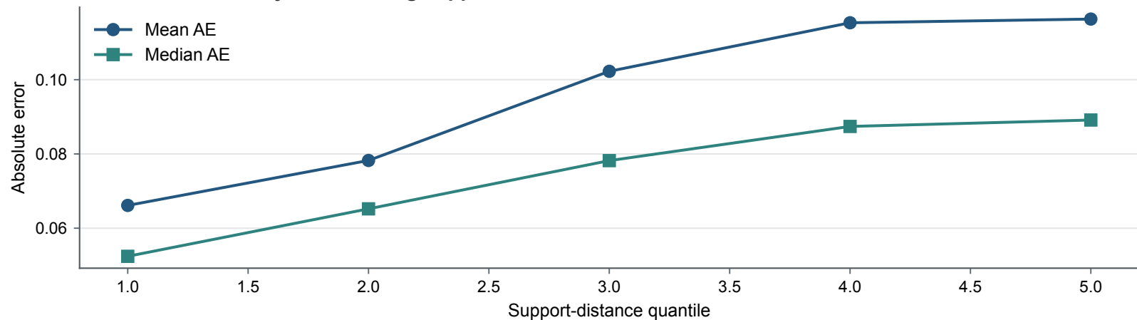
B Observation-level error by support
