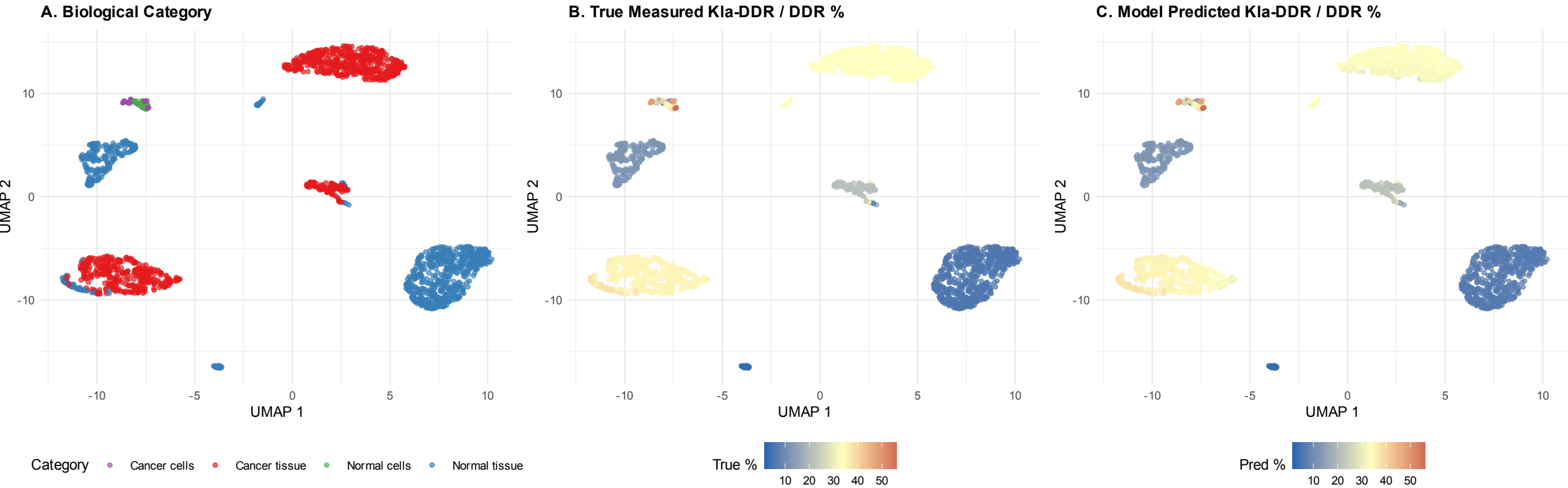
Figure 3: Transcriptomic Manifold Embedding (UMAP) Across 1,898 RNA Samples ( Kla-DDR / DDR )
