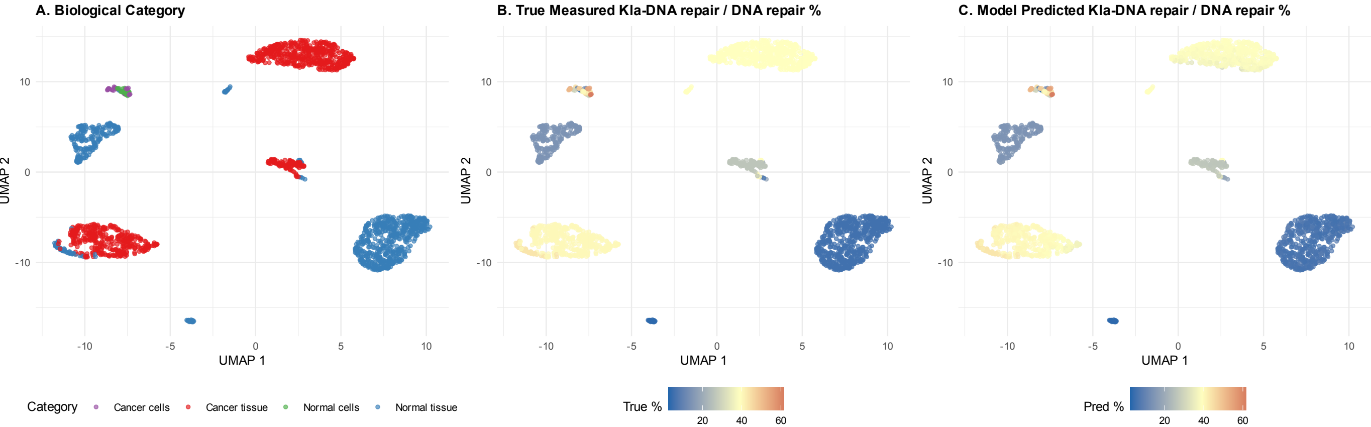
Figure 3: Transcriptomic Manifold Embedding (UMAP) Across 1,898 RNA Samples ( Kla-DNA repair / DNA repair )
