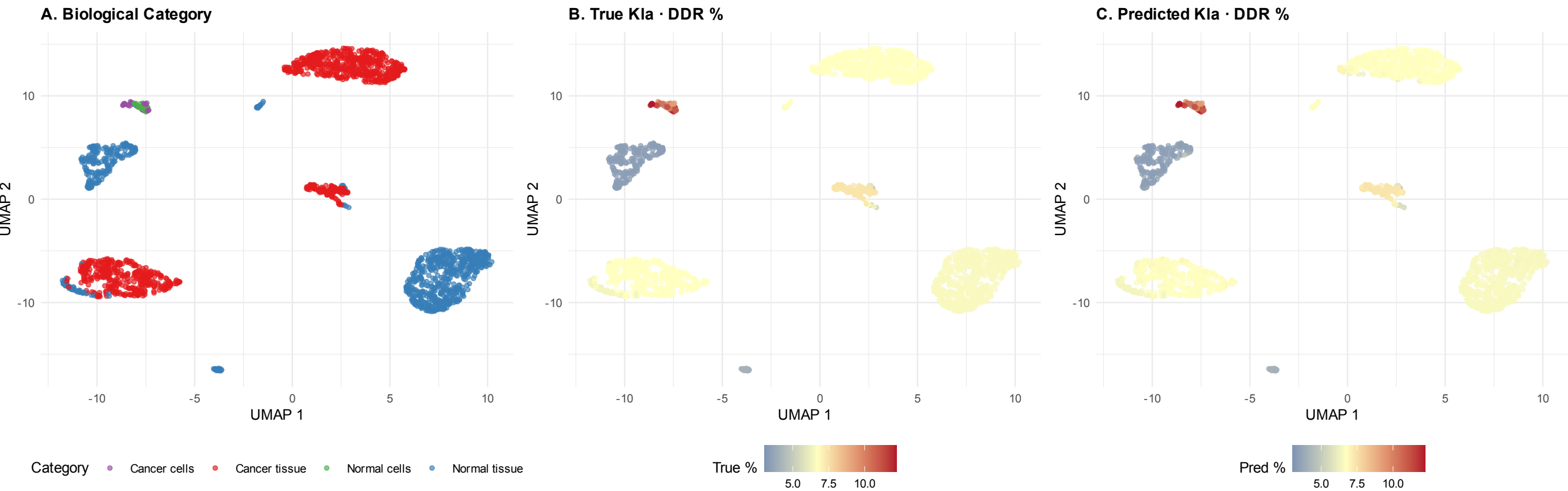
Figure 3: Transcriptomic Manifold Embedding (UMAP) Across 1,898 RNA Samples (Kla · DDR %)
