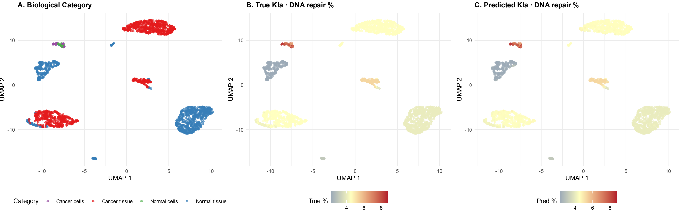
Figure 3: Transcriptomic Manifold Embedding (UMAP) Across 1,898 RNA Samples (Kla · DNA repair %)
