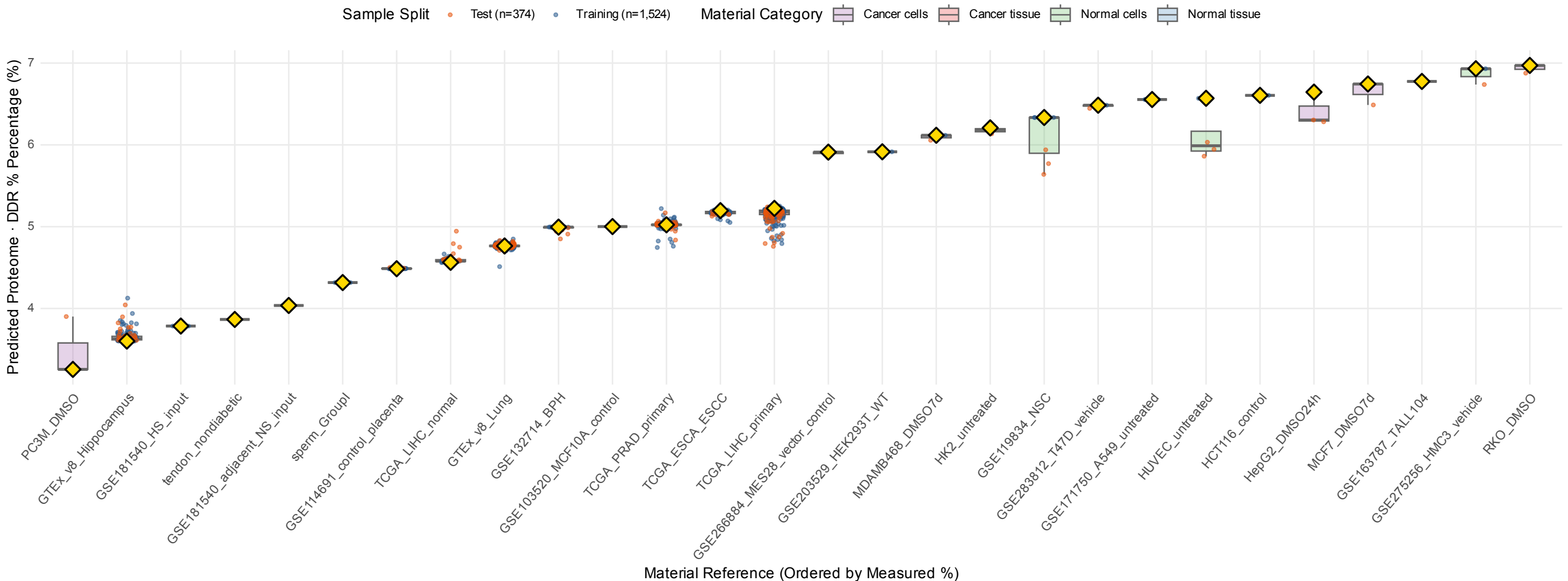
Figure 1: Individual RNA Sample Predictions vs Shared Material Labels (Proteome · DDR %)
