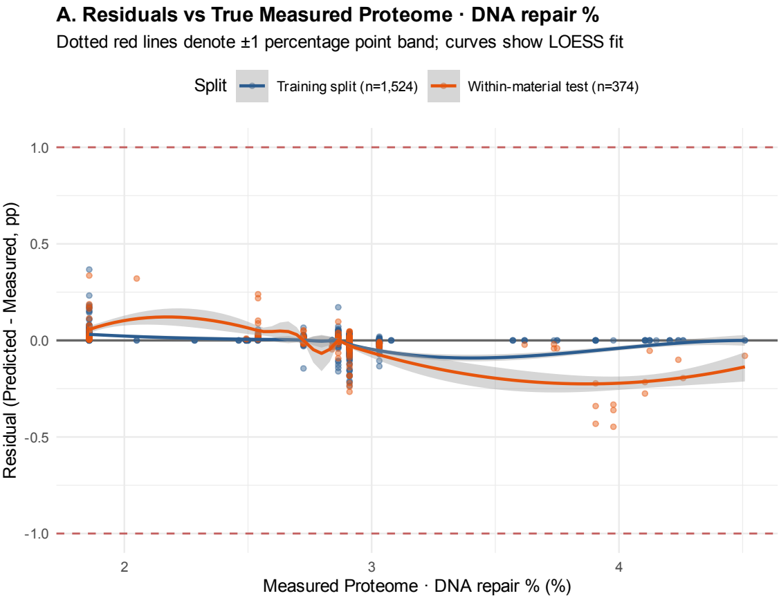
Figure 4: Model Residual Diagnostics on Training and Test Splits (Proteome · DNA repair %)
