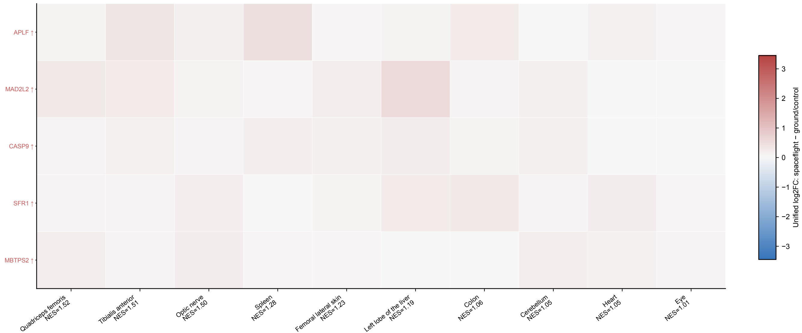
D | NES > 1, excluding Kidney Top 30 pooled genes; common direction (up 5, down 0)
