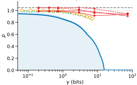
CelebA, LPIPS
