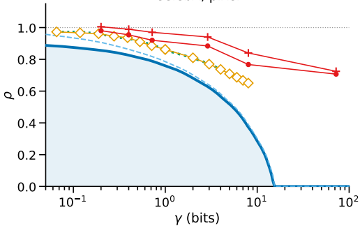
CelebA, pixel
