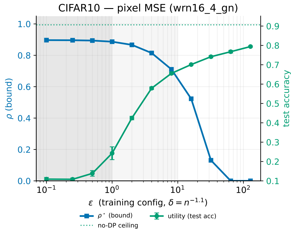
Bound vs utility — MSE
