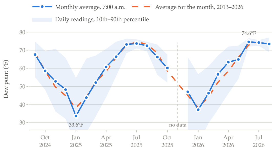
Figure 1: Monthly average 7:00 a.m. dew point at Coulter Field, Bryan, Texas, September 2024 through August 2026. The shaded band is the 10th to 90th percentile of the individual daily 7:00 a.m. readings within each month, not an uncertainty interval about the mean. November 2025 is absent because the station reported on only five days that month.
