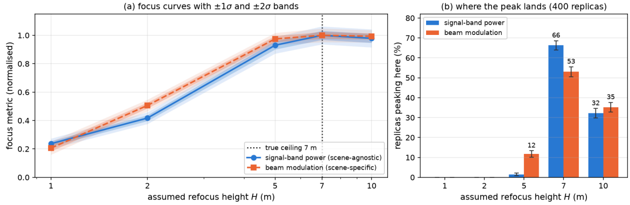
Figure 3. Scene-specific versus scene-agnostic single-detector focus, with counting-statistics uncertainty from a 400-replica Poisson bootstrap. (a) Both metrics against the assumed refocus height, normalised to their own peak, with \pm 1\sigma and \pm 2\sigma bands. Both rise steeply out of 1 m and then saturate above \sim 5 m, where the height-to-height differences are comparable to the bands themselves. (b) Which height each replica peaks at (binomial errors). The true 7.0 m ceiling wins about two-thirds of replicas for the scene-agnostic metric and about half for the scene-specific one, with most of the rest at 10 m — single-detector refocusing prefers the right height rather than measuring it.
