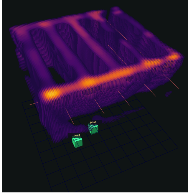
Figure 5. Voxel-cloud rendering of the full-volume reconstruction in the interactive viewer (per-voxel colour encodes opacity density; support taper applied). The five parallel beams and the brighter transverse beam are reproduced at the model-free verified positions (red guide lines); the two detectors are shown on the floor (green, pos0/pos1 ). The curtain-like veils descending below the beam grid are not structure: they visualise the depth degeneracy of Sec. 6 — opacity that the two-view geometry cannot localise in height, smeared along the viewing directions.
