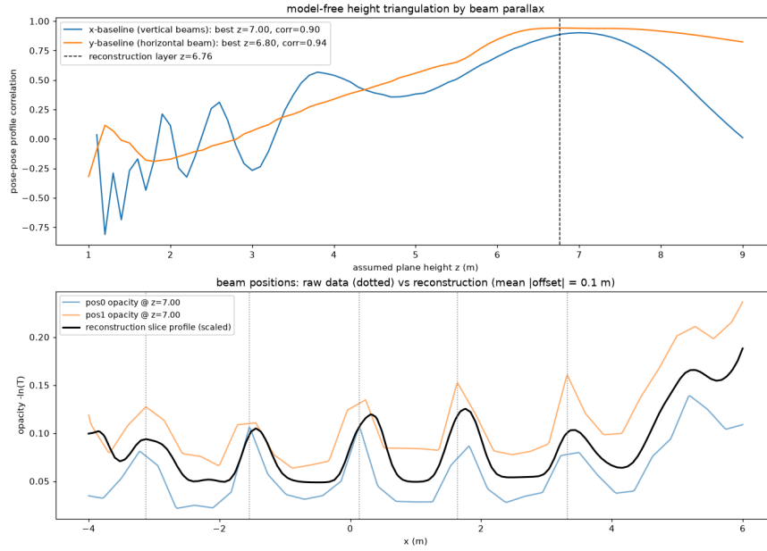
Figure 2. Model-free beam verification of run production. Top: 1-D beam-parallax height triangulation — correlation of the two detectors’ world-projected beam profiles versus assumed height; the x-baseline (across the five parallel beams) peaks at 7.0 m and the y-baseline (transverse beam) at 6.8 m, independently confirming the cross-validation autofocus of Fig. 1. Bottom: the two detectors’ measured opacity profiles back-projected at z = 7.0 m (verified beam positions dotted) overlaid with the reconstruction slice profile: all five beams are recovered with a mean position offset of 0.10 m — the verification gate every reconstruction product must pass.
