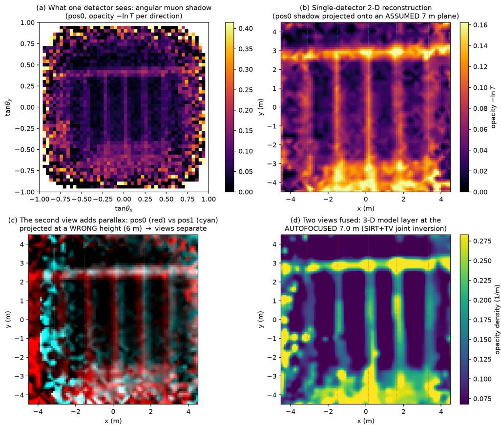
Figure 4. From one detector to two. (a) The raw measurement of a single detector: an angular opacity map in tangent space — a muon shadow with no depth information. (b) The same shadow back-projected onto an assumed 7 m plane: a clean 2-D heat-map “reconstruction” of the ceiling, but one that would look equally plausible at any other assumed height (verified beam positions dotted). (c) Adding the second detector: both shadows projected at a deliberately wrong height (6 m) separate into red (pos0) / cyan (pos1) ghost pairs — the parallax that encodes height; at the true 7.0 m they register (Fig. 1). (d) The two views jointly inverted through the physics model at the autofocused height: the ceiling layer of the 3-D voxel model, with metric height, fused statistics and verified beam positions (red dotted).
