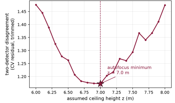
Figure 1. Autofocus on the measured data: disagreement between the two detectors (cross-validation prediction residual, worst-10% of bins trimmed) versus assumed ceiling height, scanned at 0.1 m steps. The smooth single minimum selects z = 7.0 m.
