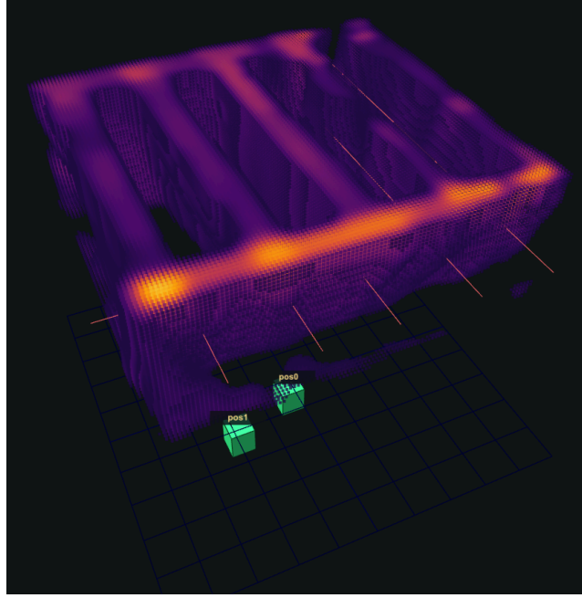
Figure 4. Voxel-cloud rendering of the full-volume reconstruction in the interactive viewer (per-voxel colour encodes opacity density; support taper applied). The five parallel beams and the brighter transverse beam are reproduced at the model-free verified positions (red guide lines); the two detectors are shown on the floor (green, pos0/pos1 ). The curtain-like veils descending below the beam grid are not structure: they visualise the depth degeneracy of Sec. 6 — opacity that the two-view geometry cannot localise in height, smeared along the viewing directions.
