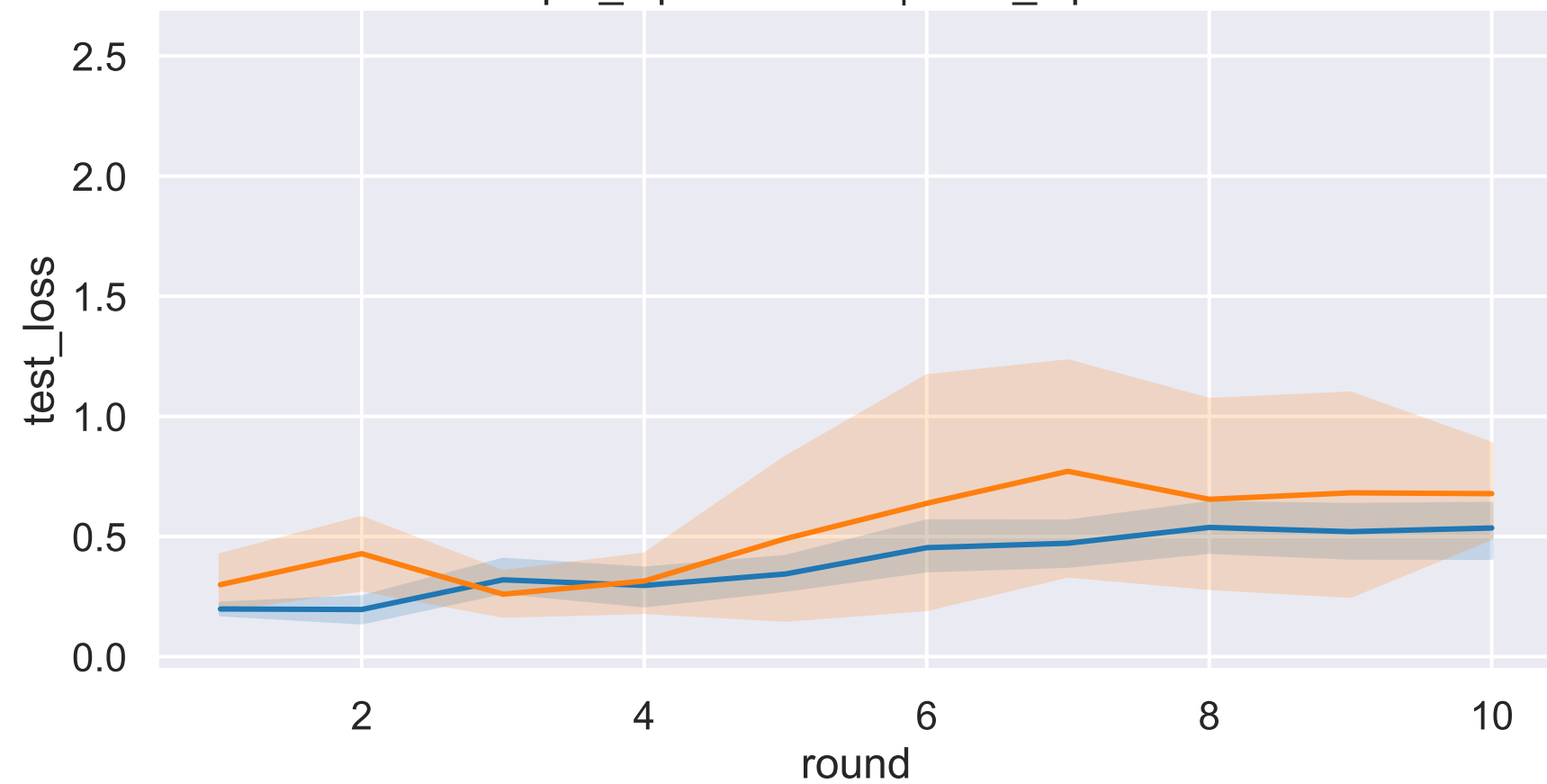
sample_alpha = 100.0 | label_alpha = 1.0
