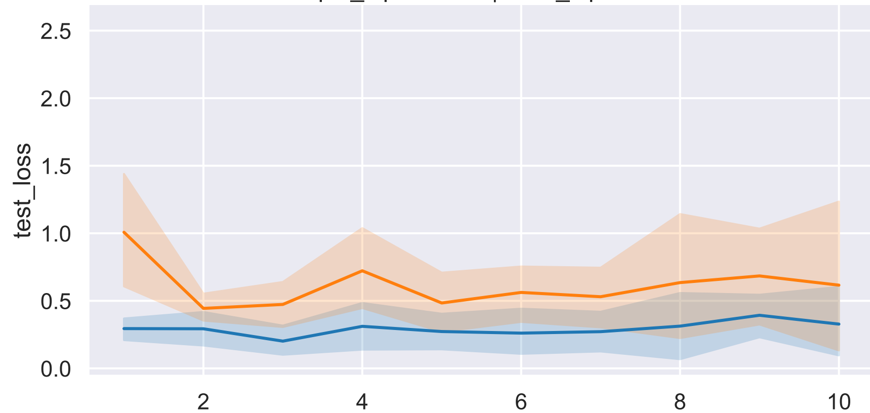
sample_alpha = 1.0 | label_alpha = 1.0
