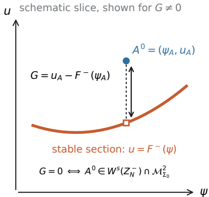
(b) Defining function on \mathcal{M}_{\Sigma_0}^2
