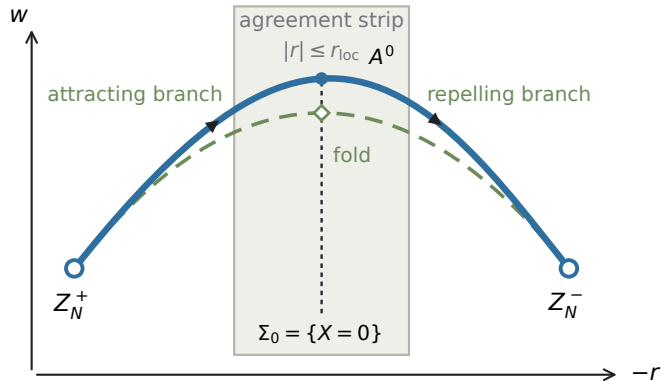
(a) Projection at G = 0
