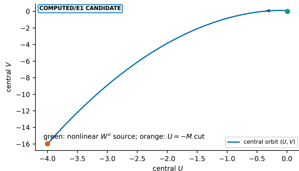
(c) same candidate on the finite outer graph
