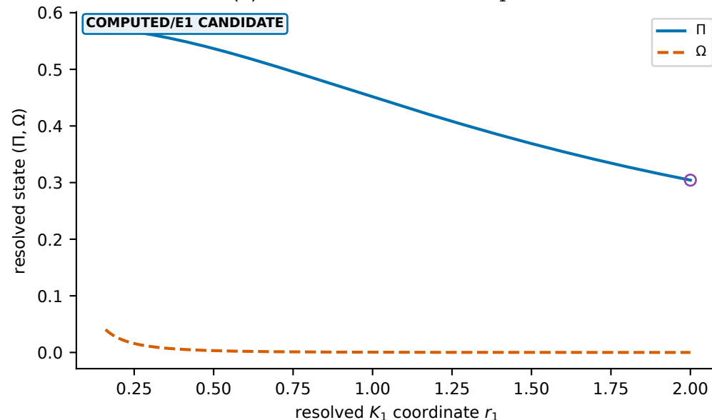
(d) finite diagnostics versus unfinished theorem objects
