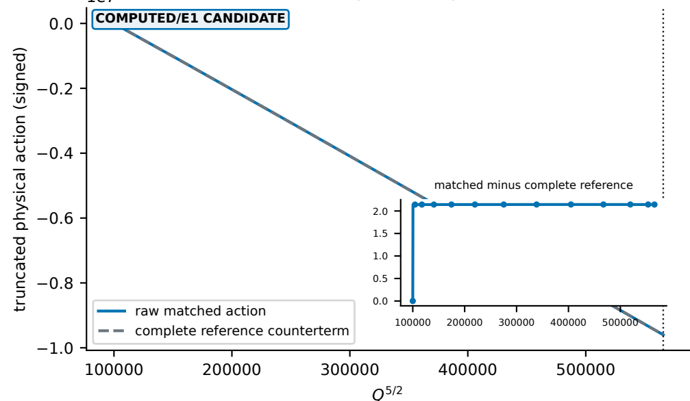
(c) raw action and negative complete counterterm
