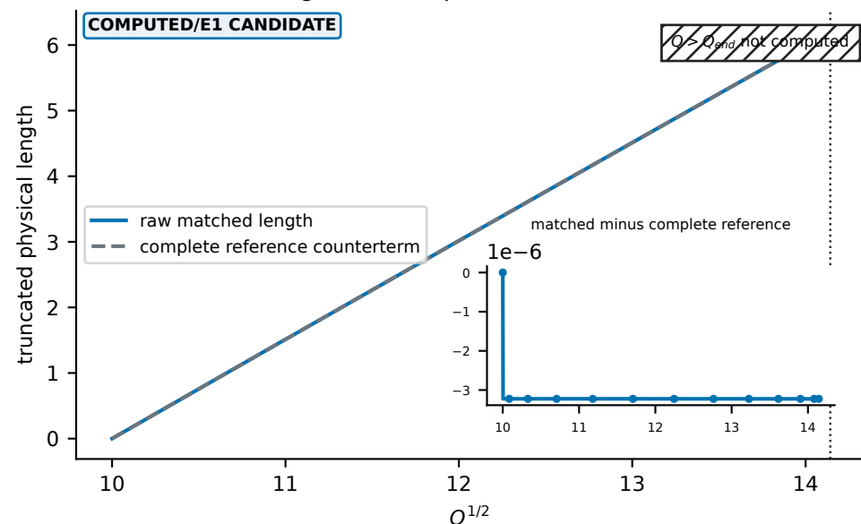
(d) cutoff, grid, horizon, and bookkeeping
