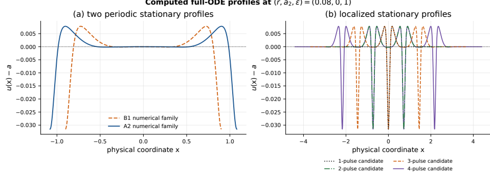
FIGURE 2. COMPUTED/E1. Finite-domain numerical candidates for stationary profiles of the original van der Pol PDE at (r, a_2, \epsilon) = (0.08, 0, 1) . (a) Two full-ODE periodic candidates, distinguished by both color and line style. (b) Full-ODE one- through four-pulse homoclinic candidates reconstructed in the physical coordinate. All curves show u - a ; the dotted horizontal line is the homogeneous state. The periodic candidates have closure, energy, step-refinement, and stationary-residual checks; the localized candidates have collocation, boundary, tail, energy, and stationary-residual checks, all archived with the numerical atlas. The family and pulse-count labels in this panel are numerical labels, not certified V6/V7 edge itineraries. The figure is non-claim-bearing and makes no temporal-stability, Turing-selection, or canard claim.
