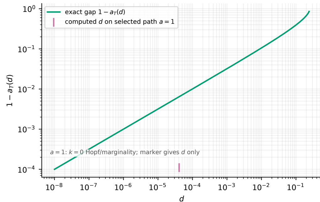
Application chain: atlas reaches stationary-profile stage
