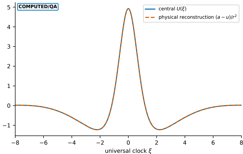
(c) same finite orbit in two formulations
