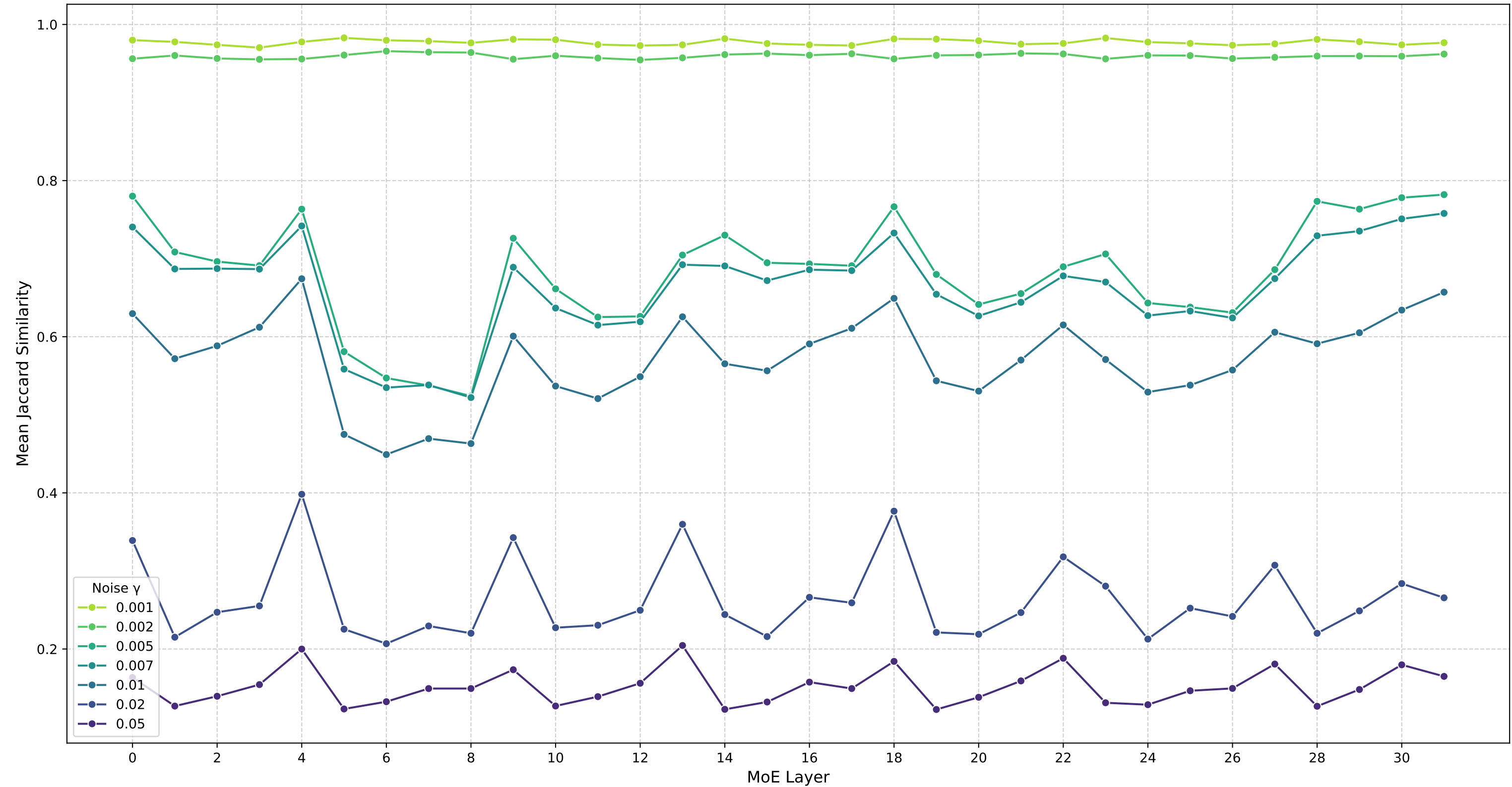
Router Stability Across Layers and Noise Levels
