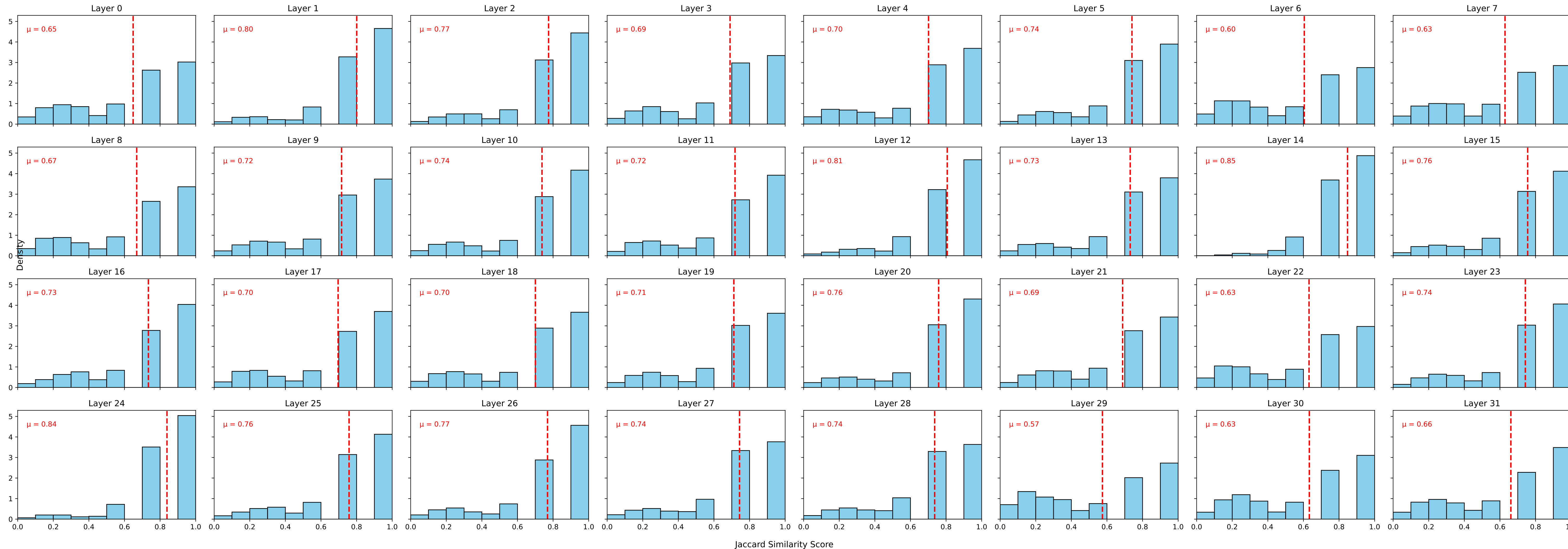
Distribution of Router Stability Under Input Perturbation
