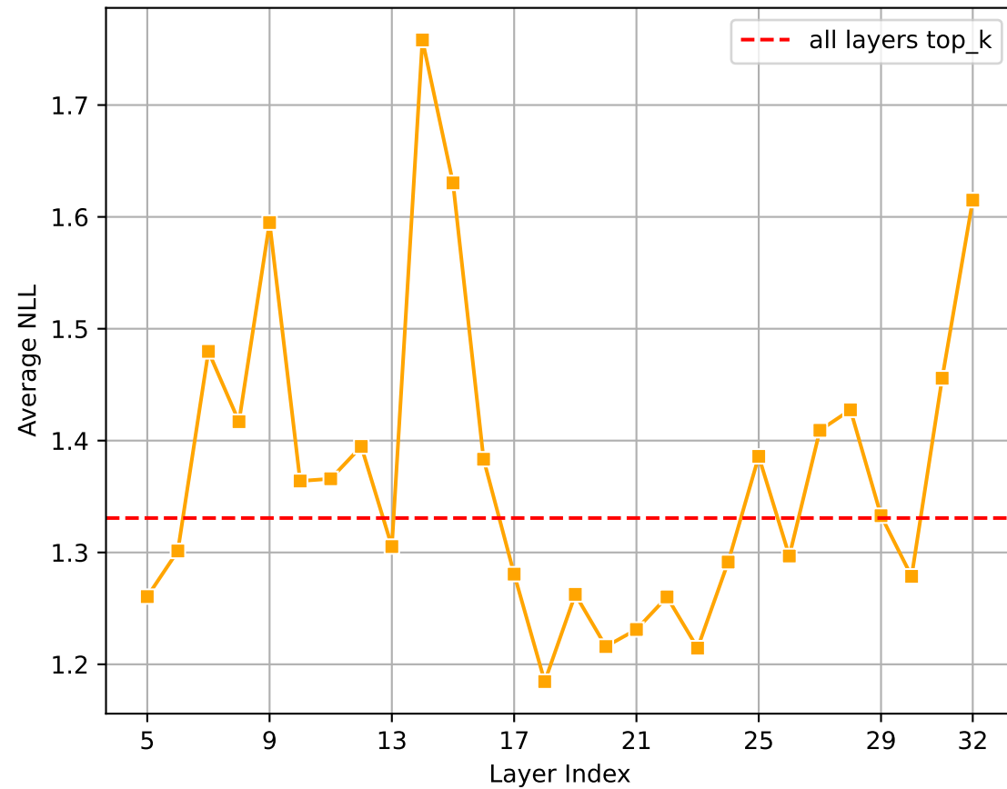
Average NLL
