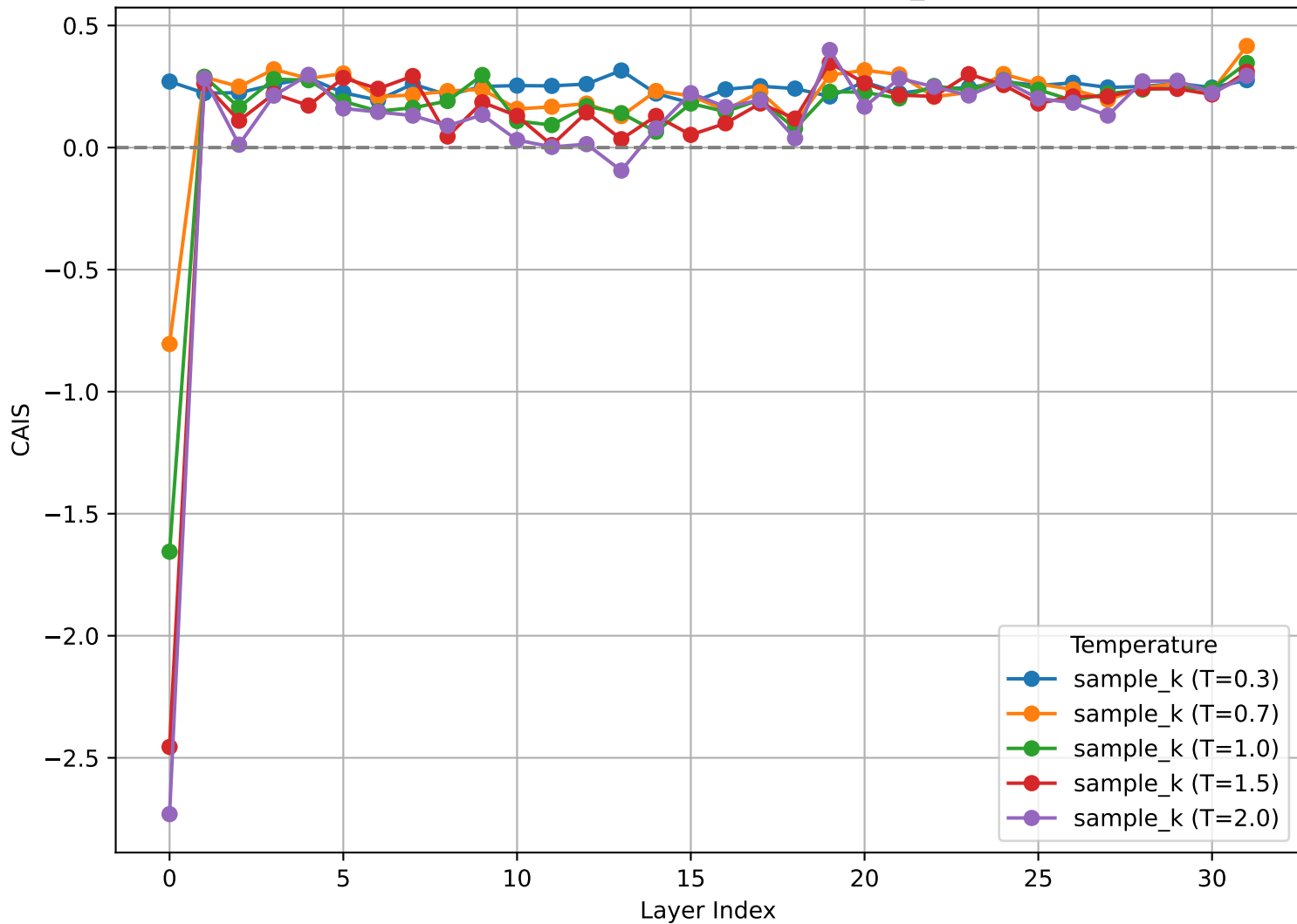
CAIS vs Layer Index for sample_k
