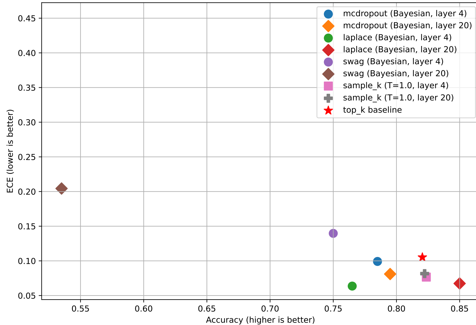
Accuracy vs ECE (ID)
