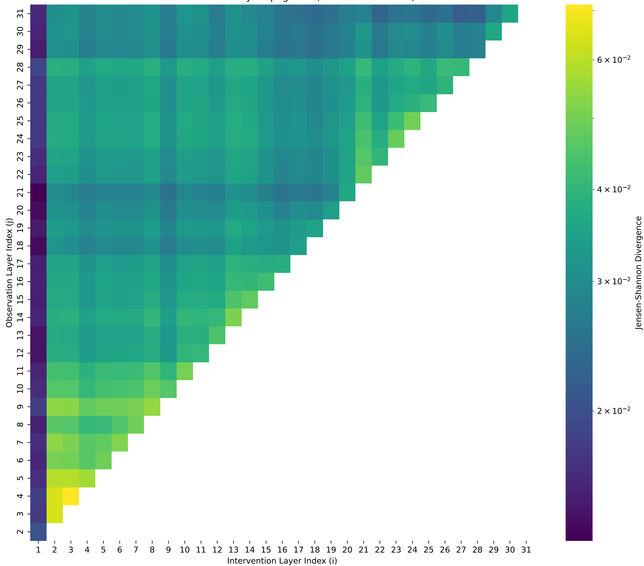
Heuristic Uncertainty Propagation (Intervention T=1.0)
