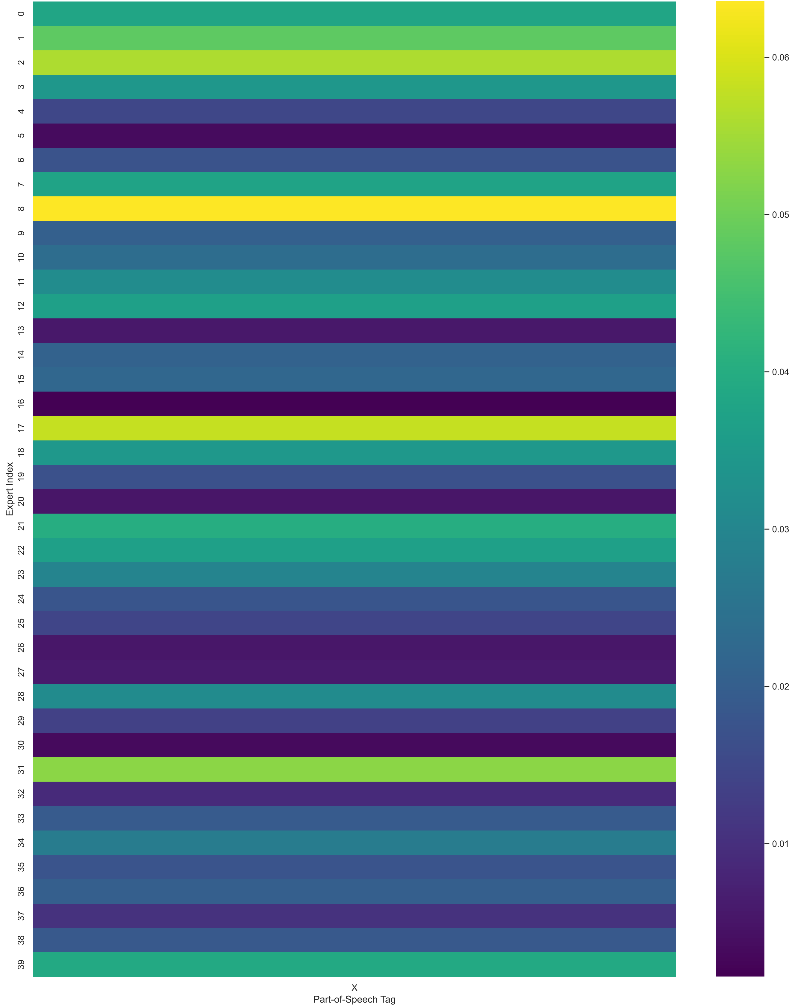
Expert Activation Probability given Part-of-Speech Tag (Layer 20)
