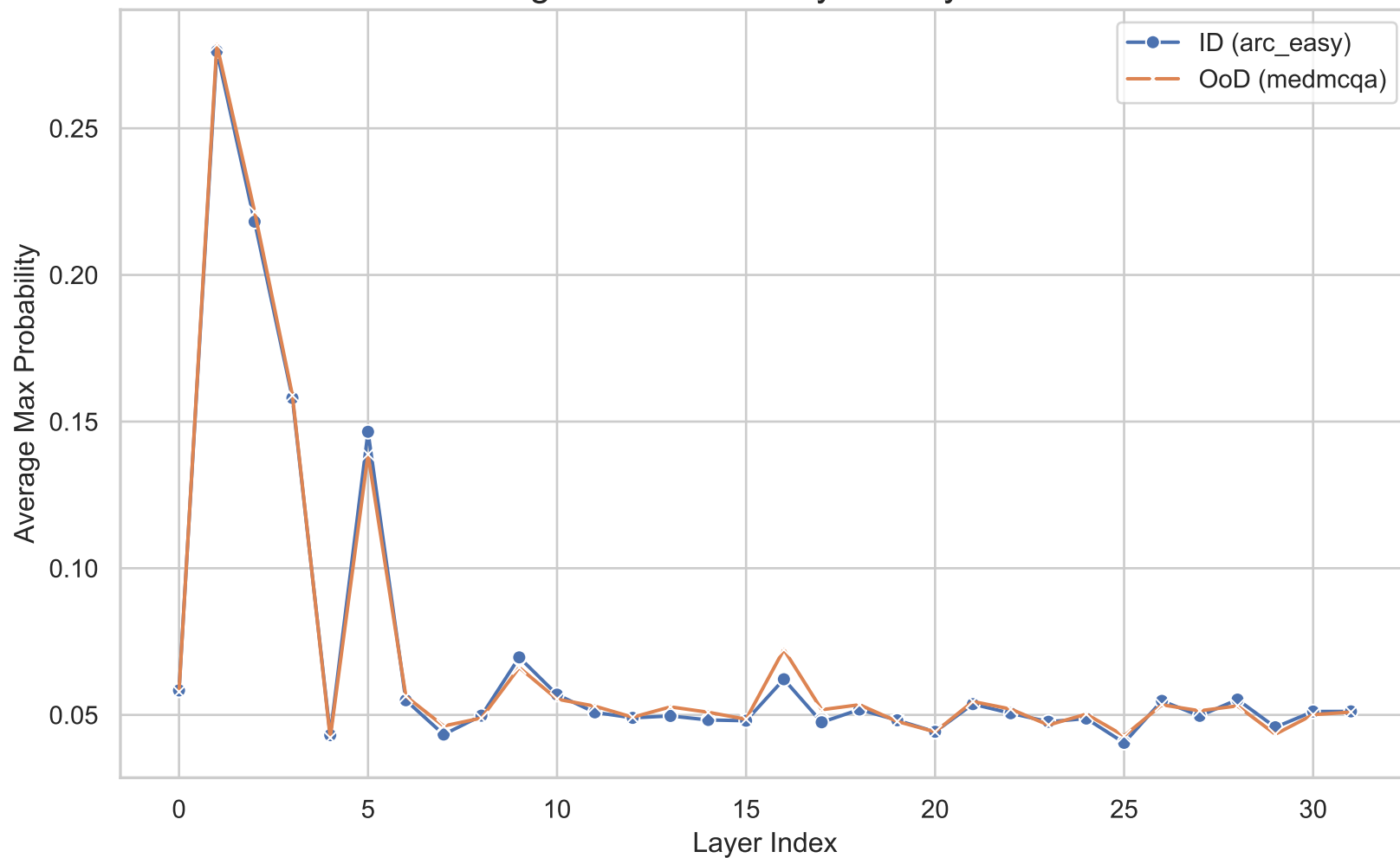
Average Max Probability vs. Layer Index
