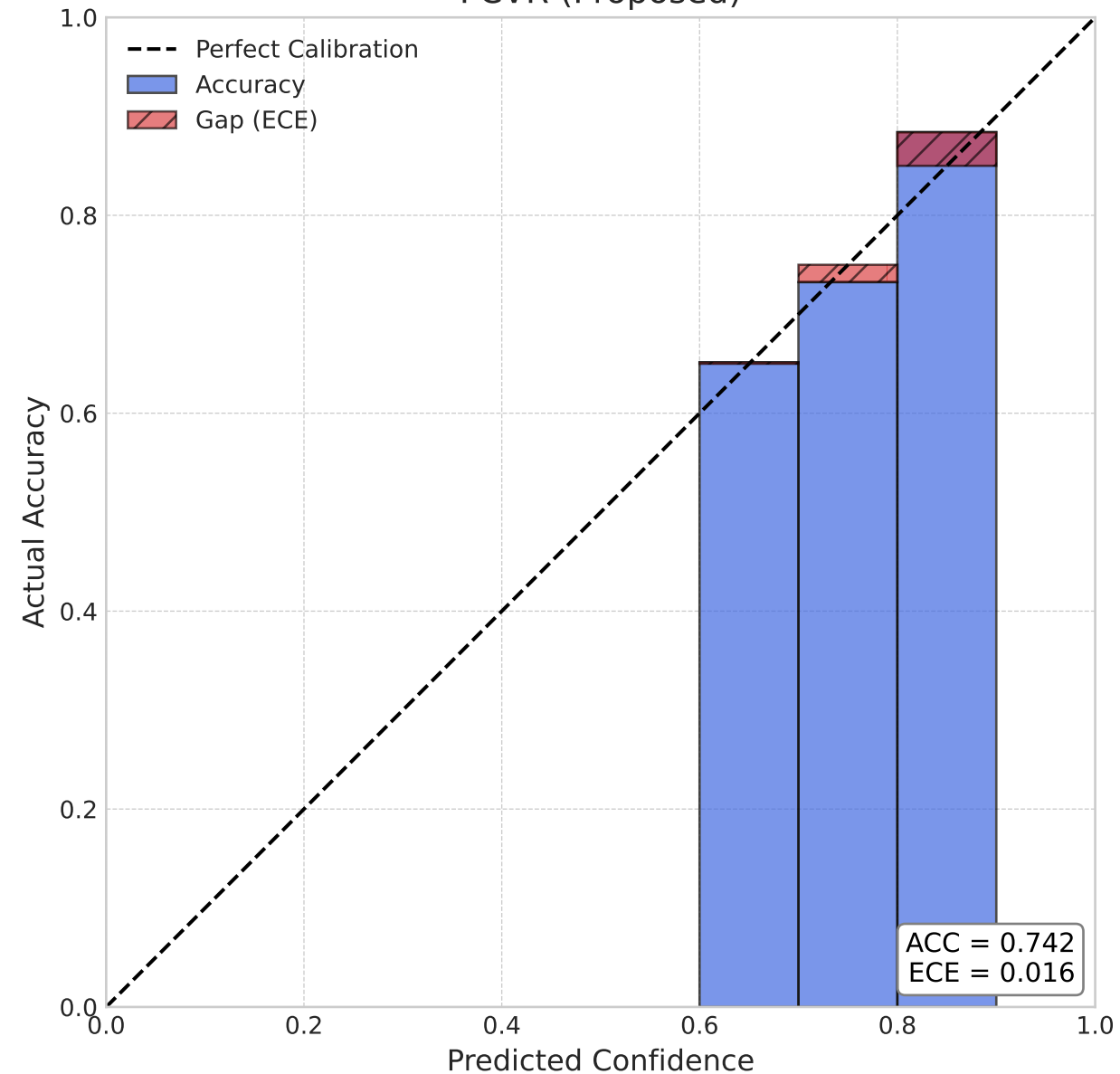
FCVR (Proposed)
