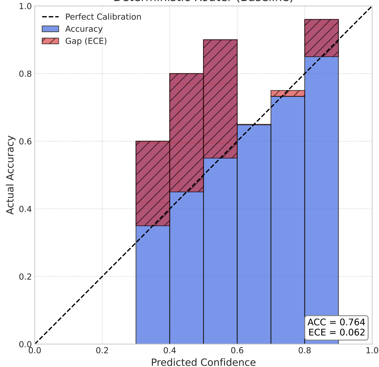
Deterministic Router (Baseline)
