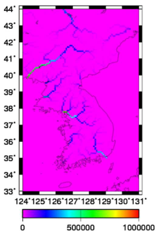
Figure 17. River discharge ( \text{kg s}^{-1} )
