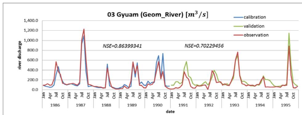
Figure 33. River discharge of Gyum in the Geom River
