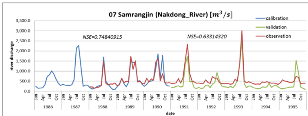
Figure 37. River discharge of Samrangjin in the Nakdong River
