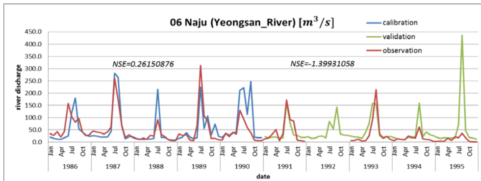
Figure 36. River discharge of Naju in the Yeongsan River
