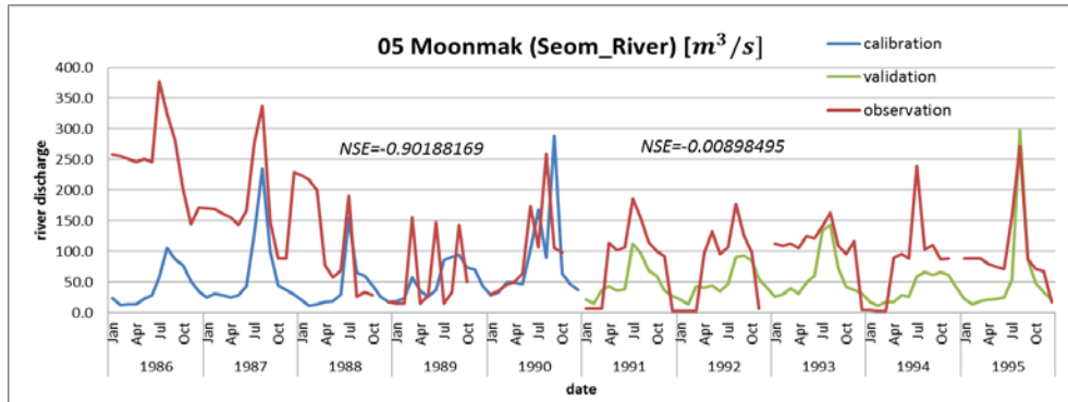
Figure 35. River discharge of Moonmak in the Seom River
