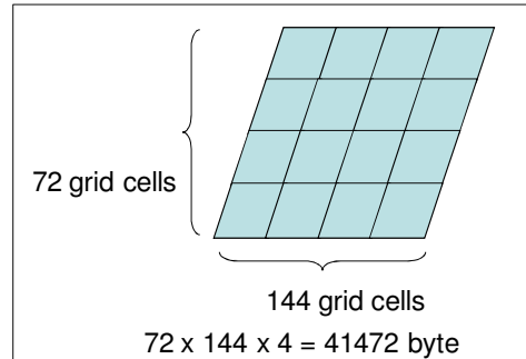
Figure 4-1 Legend for binary files of CMAP data
