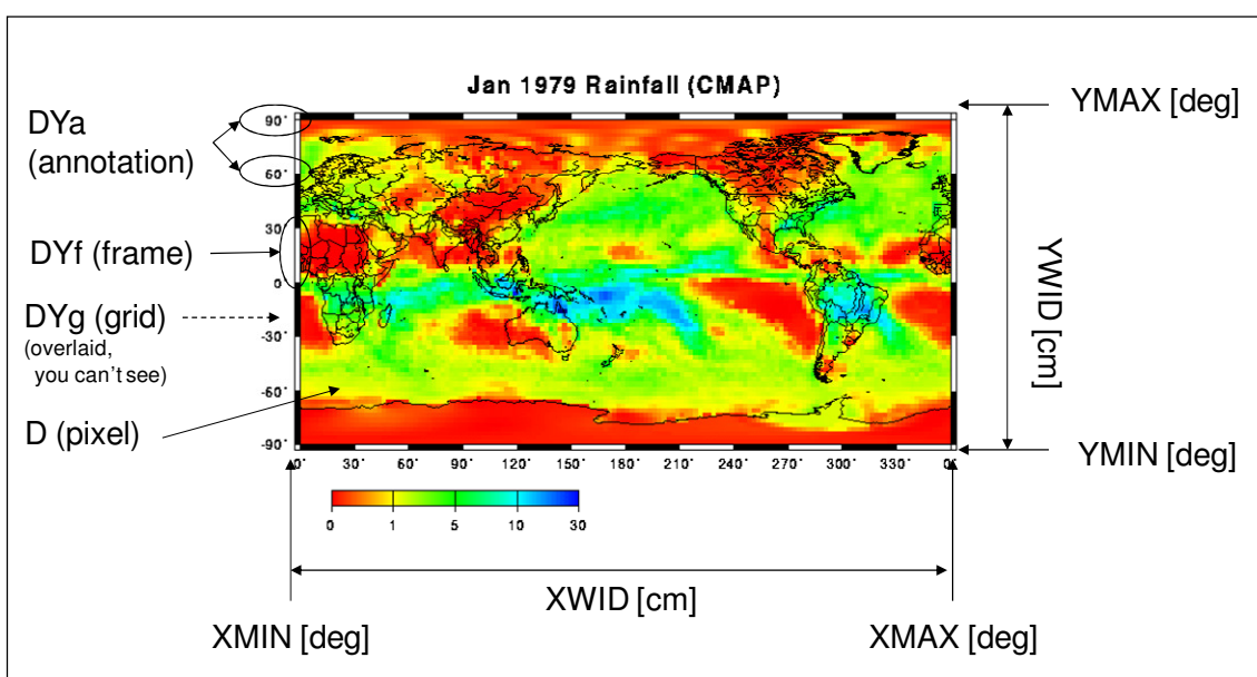
Figure 3-2 Plotting region of GMT
