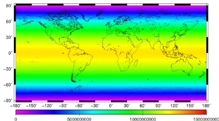
Figure 6-1 A world map of grdara.hlf [ \text{m}^2 ]
