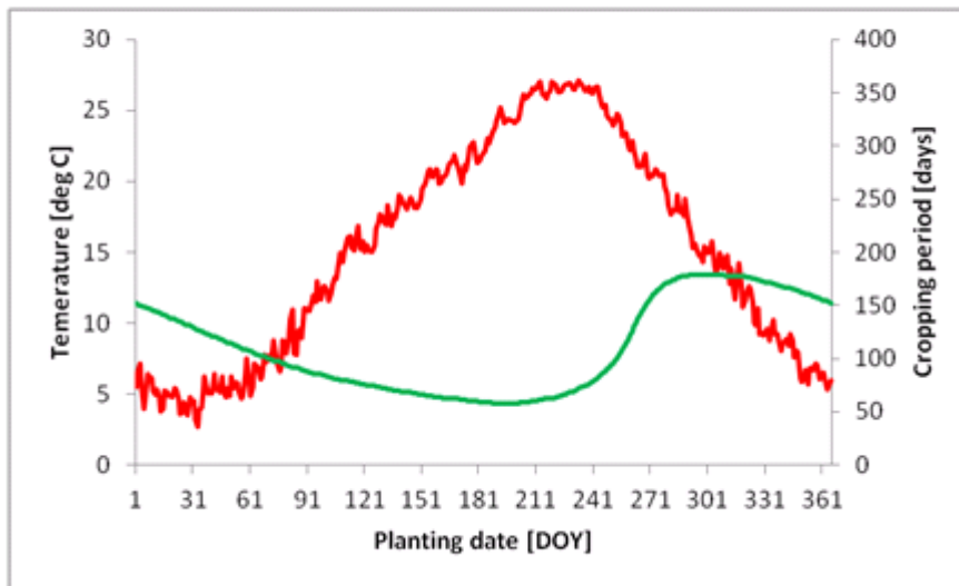
Figure 10-1. Daily average temperature [ ^{\circ}\text{C} ] (red) and cropping period [days] (green) for an imaginary location
