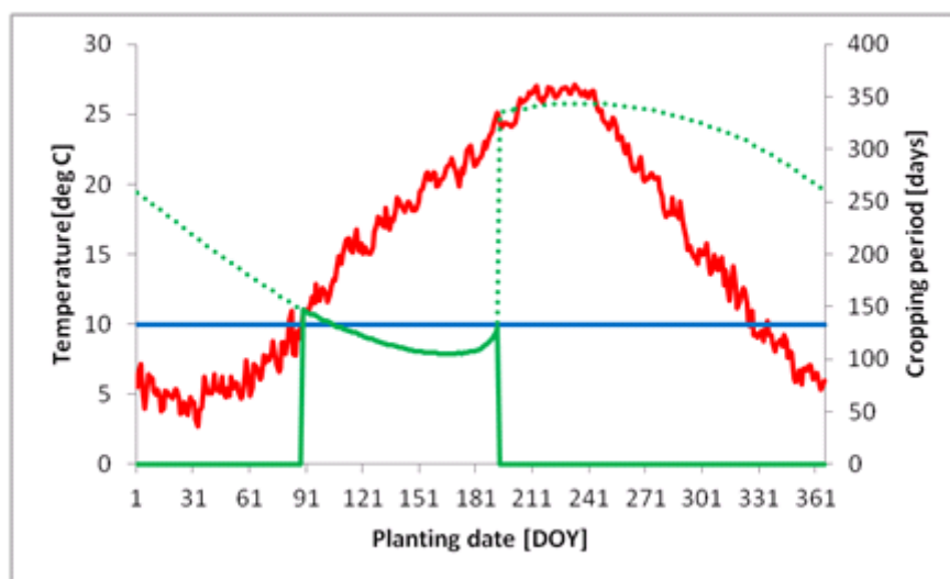
Figure 10-2. Daily average temperature [ ^{\circ}\text{C} ] (red) and cropping period [days] (green) with effective accumulative temperature
