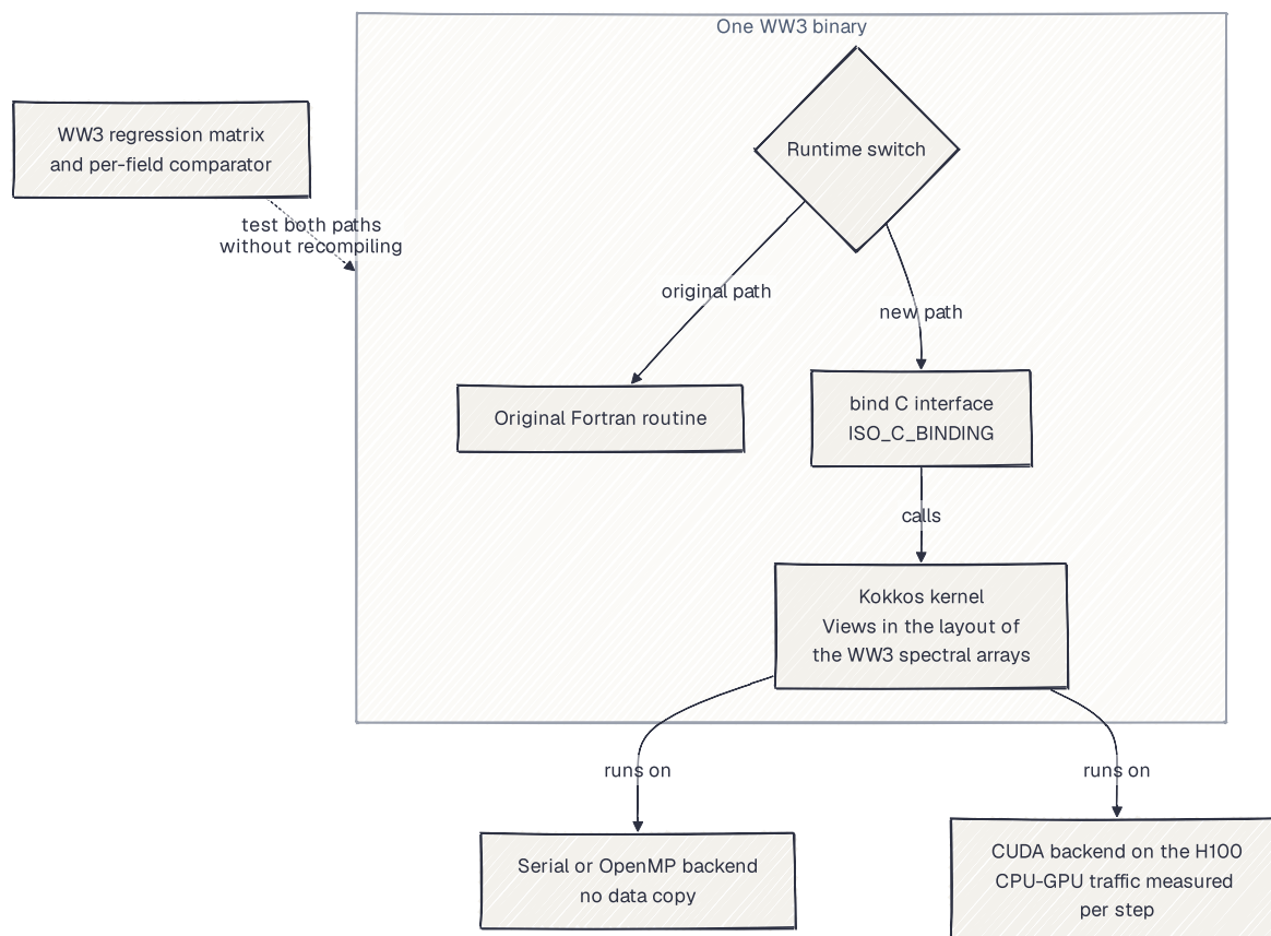
Figure 14.2: How do the original Fortran routine and its Kokkos kernel coexist in one WW3 binary?
