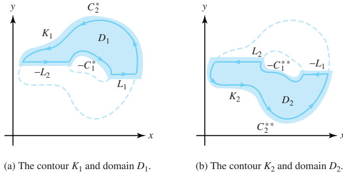
Figure 6.23: The cuts L_1 and L_2 and the contours K_1 and K_2 used to prove the deformation of contour theorem
