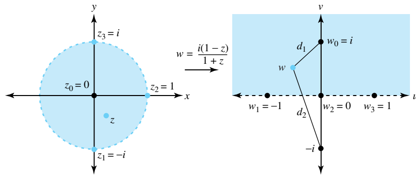
Figure 9.5: The image of |z| < 1 under w = \frac{i(1-z)}{1+z}
