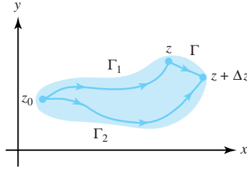
Figure 6.30: The contours \Gamma_1 and \Gamma_2 and the line segment \Gamma
