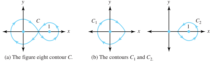
Figure 6.27: The contour C = C_1 + C_2
