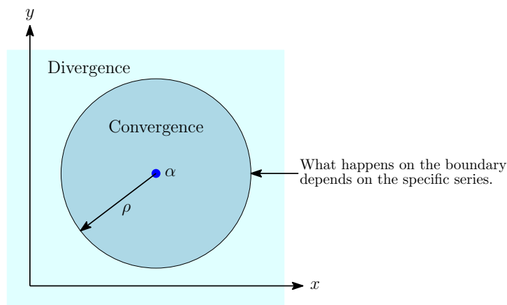
Figure 4.8: The radius of convergence of a power series
