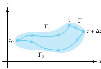
Figure 6.30: The contours \Gamma_1 and \Gamma_2 and the line segment \Gamma
