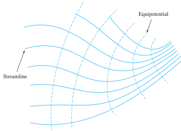
Figure 3.4: The families of orthogonal curves \{(x, y) : \phi(x, y) = \text{constant}\} and \{(x, y) : \psi(x, y) = \text{constant}\} for the function F(z) = \phi(x, y) + i\psi(x, y)
