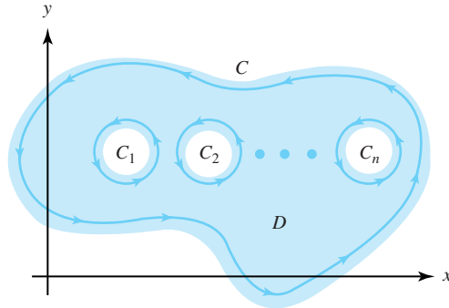
Figure 6.25: The multiply connected domain D and the contours C and C_1, C_2, \dots, C_n in the statement of the extended Cauchy-Goursat theorem
