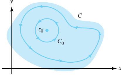
Figure 6.32: The contours C and C_0 in the proof of Cauchy's integral formula
