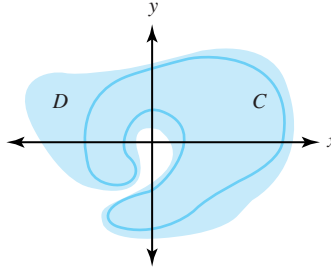
Figure 6.21: A simple connected domain D containing the simple closed contour C that does not contain the origin
