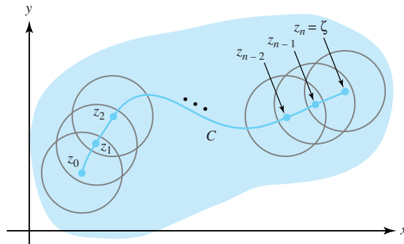
Figure 6.33: The “chain of disks” D_0, D_1, \dots, D_n that cover C
