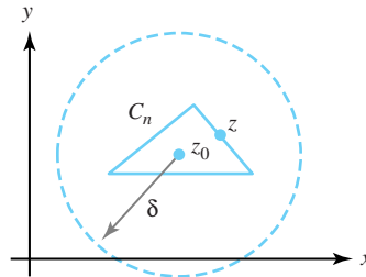
Figure 6.20: The contour C_n that lies in the neighborhood |z - z_0| < \delta
