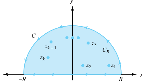
Figure 8.4: The poles of \frac{P}{Q} that lie in the upper half-plane
