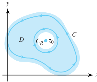
Figure 6.24: The domain D that contains both C and C_R
