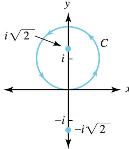
Figure 6.26: The circle C_1^+(i) and the points z = \pm i\sqrt{2}
