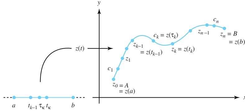
Figure 6.7: A parameterization of the contour C by z(t) , for a \leq t \leq b
