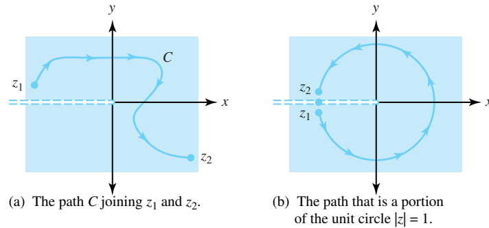
Figure 6.31: The paths C from Examples 6.19 and 6.20
