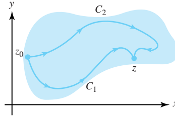
Figure 6.29: The contours C_1 and C_2 joining z_0 to z
