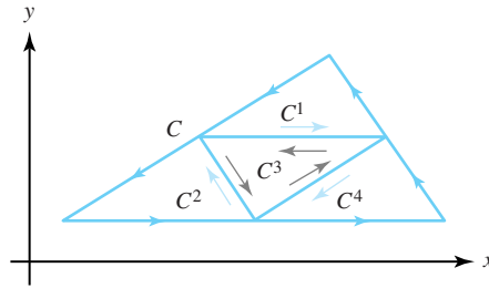
Figure 6.19: The triangular contours C and C^1 , C^2 , C^3 , and C^4
