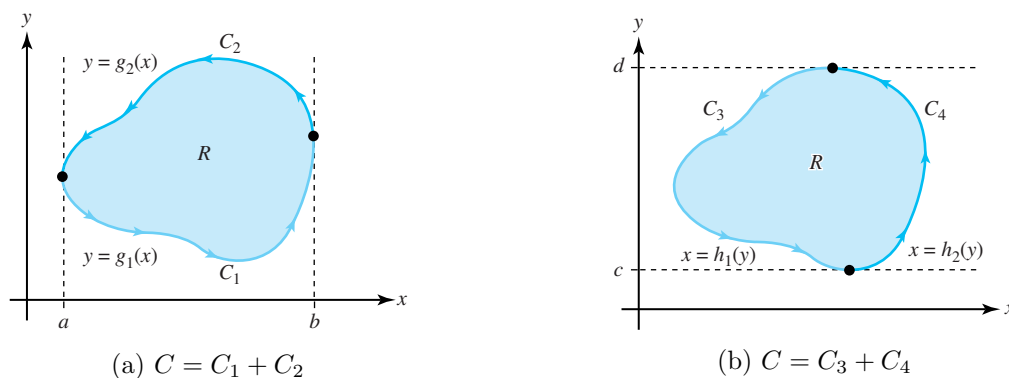
Figure 6.18: A Standard Region R
