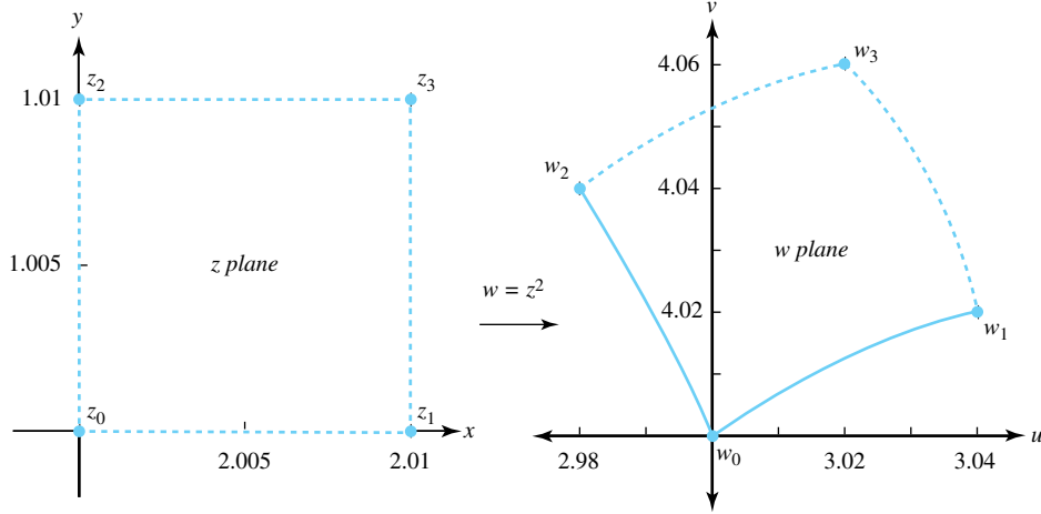
Figure 3.1: The image of a small square under w = z^2
