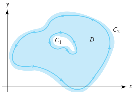
Figure 6.22: The domain D that contains the simple closed contours C_1 and C_2 and the region between them
