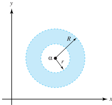
Figure 7.3: The open annulus A(\alpha, r, R)
