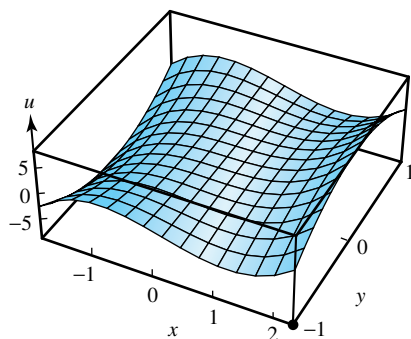
(a) u(x, y) = x^3 - 3xy^2
