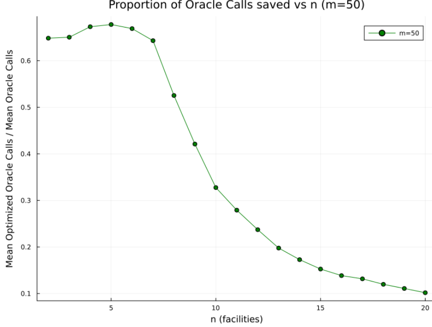
Figure 4: Proportion of oracle calls saved for different values of n
