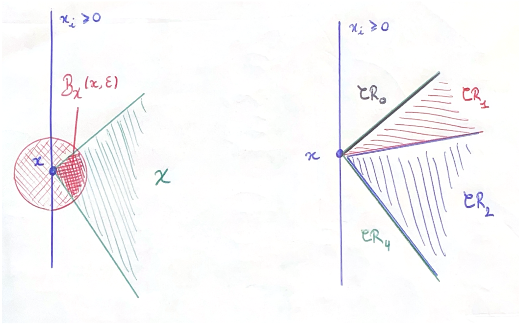
Figure 5: Illustration for part (i) and (ii) of the proof
