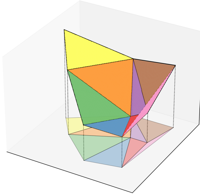
Figure 3: Visual of the recourse function with a 2d parameter
