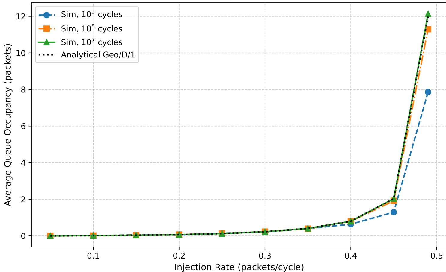
E1: Geo/D/1 occupancy vs injection rate ( S = 2 )
