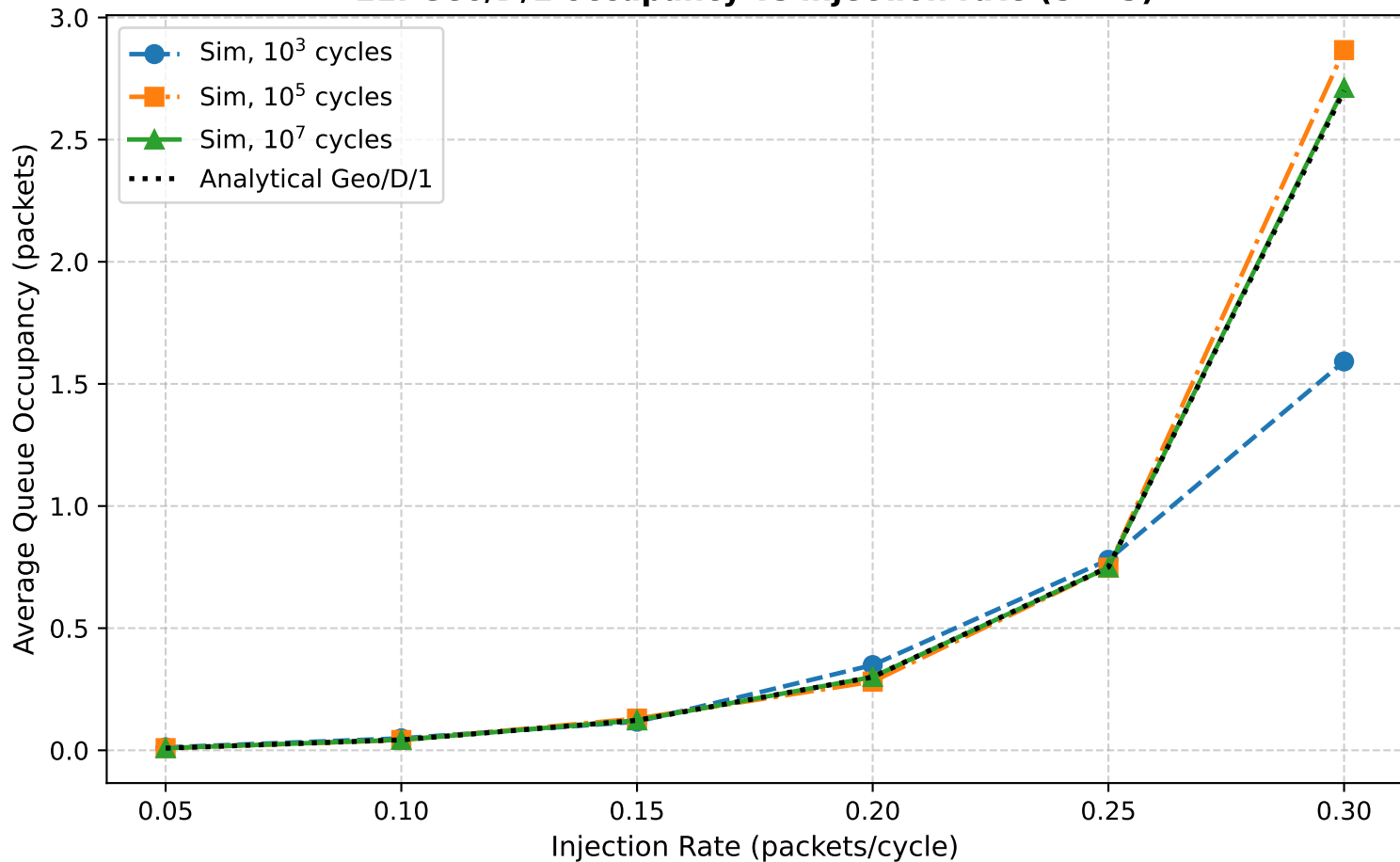
E1: Geo/D/1 occupancy vs injection rate ( S = 3 )
